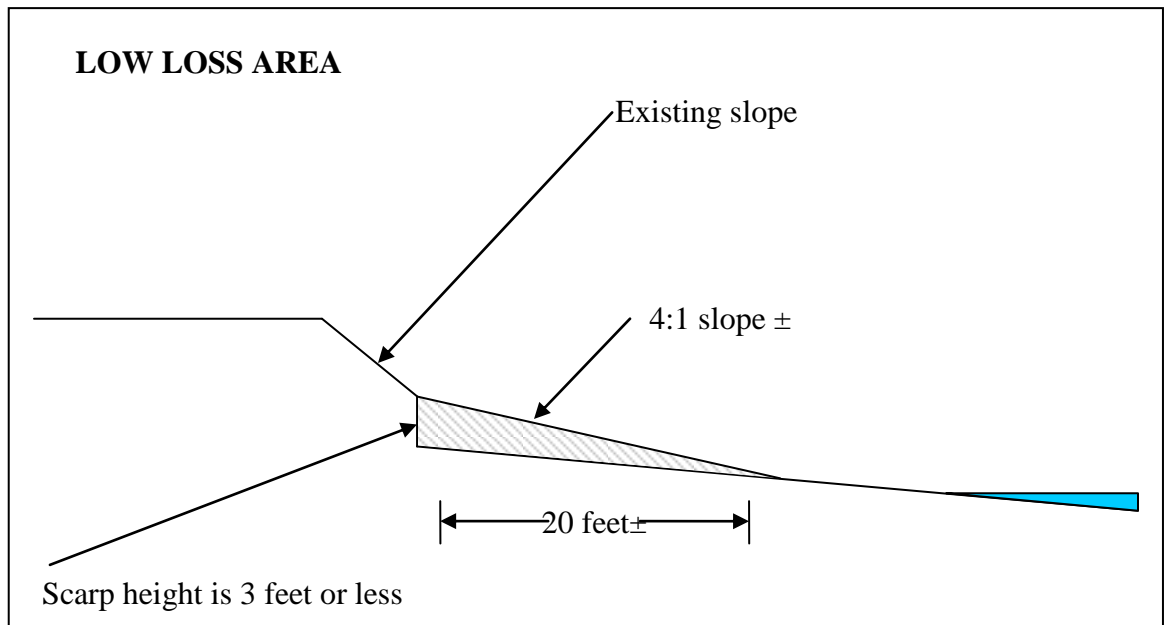
Figure 10. Recommended slope on a low erosion beach for sand placement projects that include the creation of a dune.
