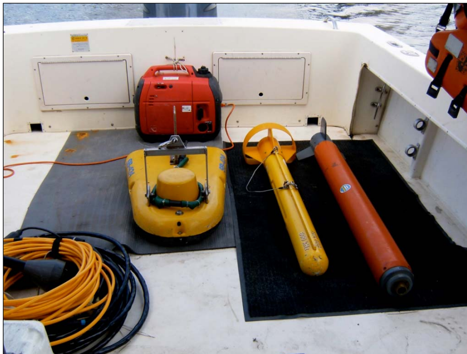
Figure 26. Survey instruments employed during the investigation included (from right to left) the magnetometer, the sidescan sonar, and the subbottom profiler. Honda generator employed to power the instruments is in the background adjacent to the transom.
